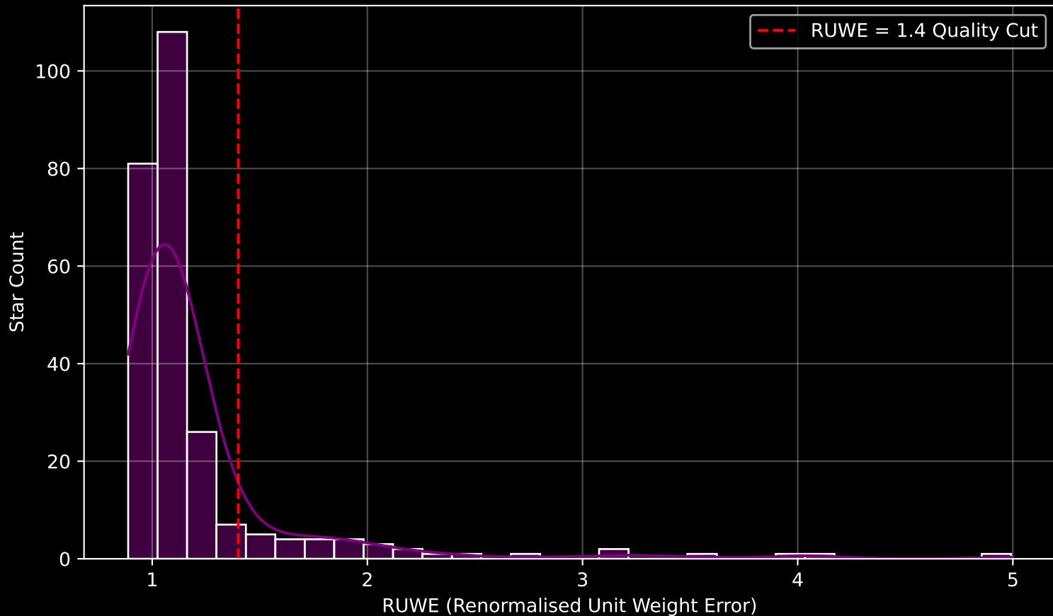
GALAH DR4 Field [8958] RUWE Distribution (n= 253)
