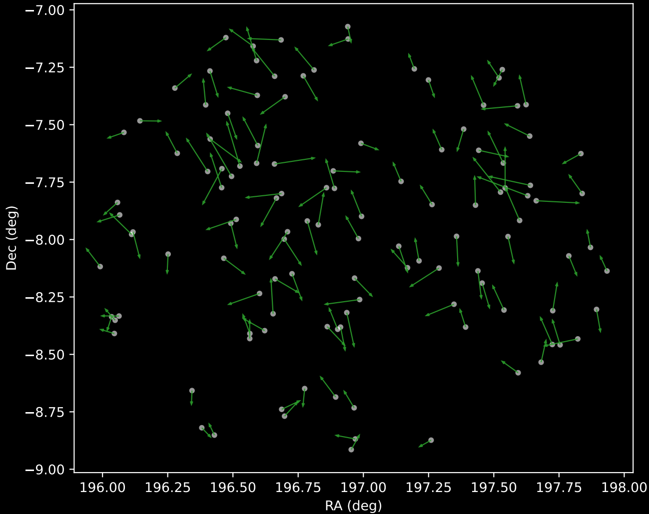
GALAH DR4 Cluster 4 Proper Motion Vectors (n=120)
