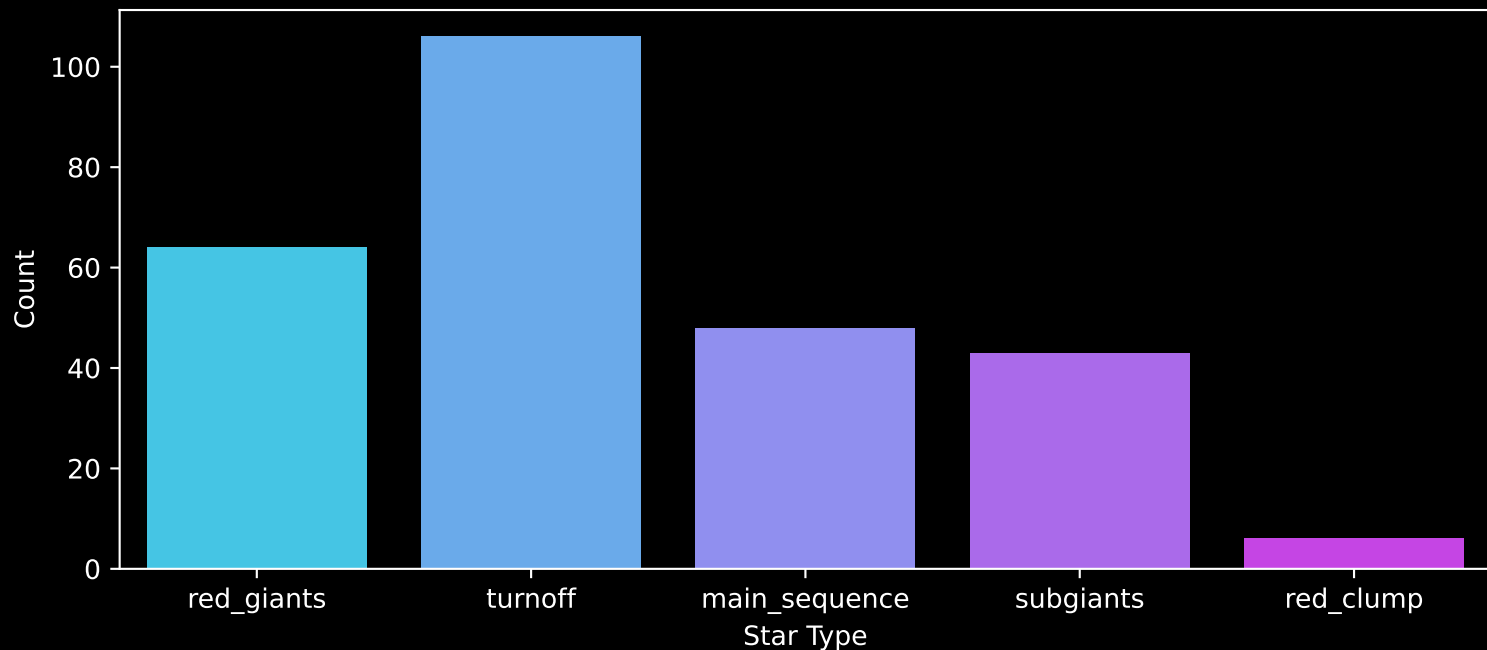
GALAH DR4 Field: [8958] Count plot of Star Type
